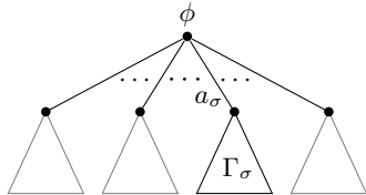
Figure 3: Structure of the auxiliary game \Gamma^* .
